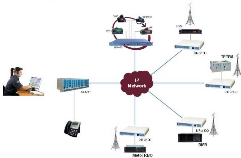
Figure 42: Typical DX-Altus Solution
