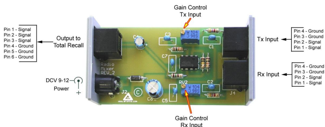
Figure 40: Radio Mixer Connectors and Pin Assignment
