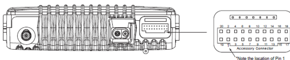
Figure 26 Location of Accessory Connector - Rear Side
