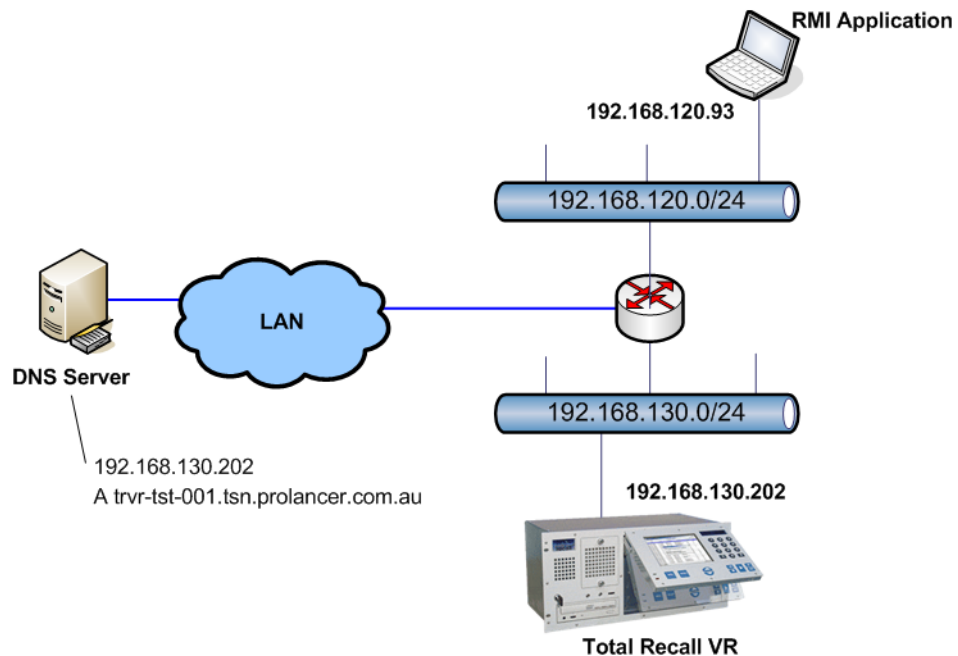
Figure 42: RMI Application using Hostname
