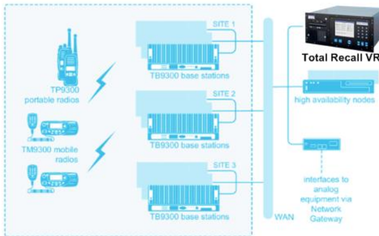
Figure 52: Tait DMR Tier 3 Solution with Total Recall VR
