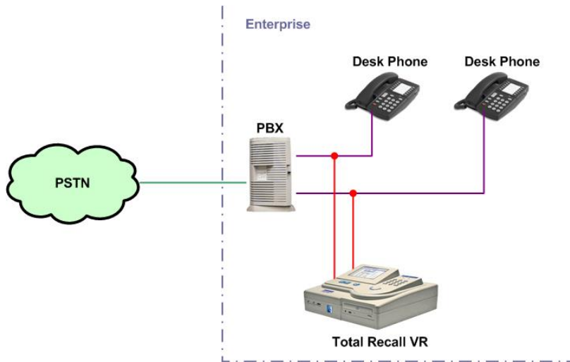
Figure 1: Extension Side Recording
