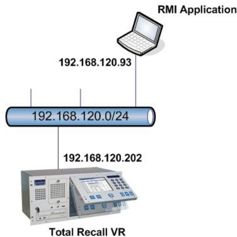
Figure 41: RMI Application using Static IP Address
