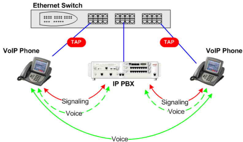
Figure 10: Media Shuffling
