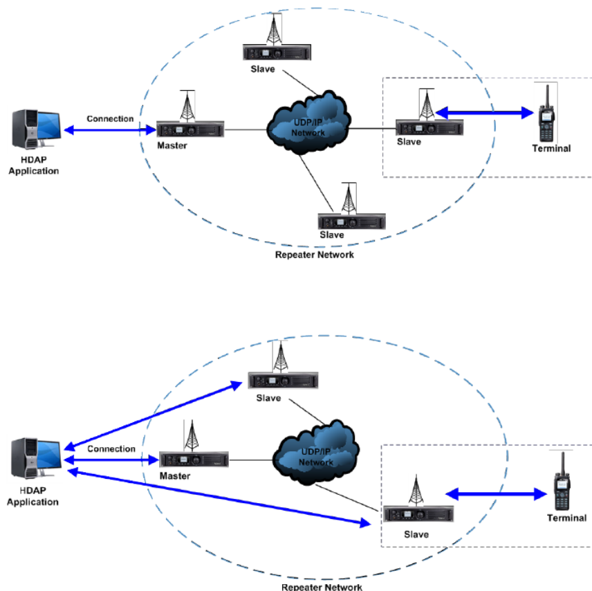
Figure 54: Example Connection to Hytera Network
