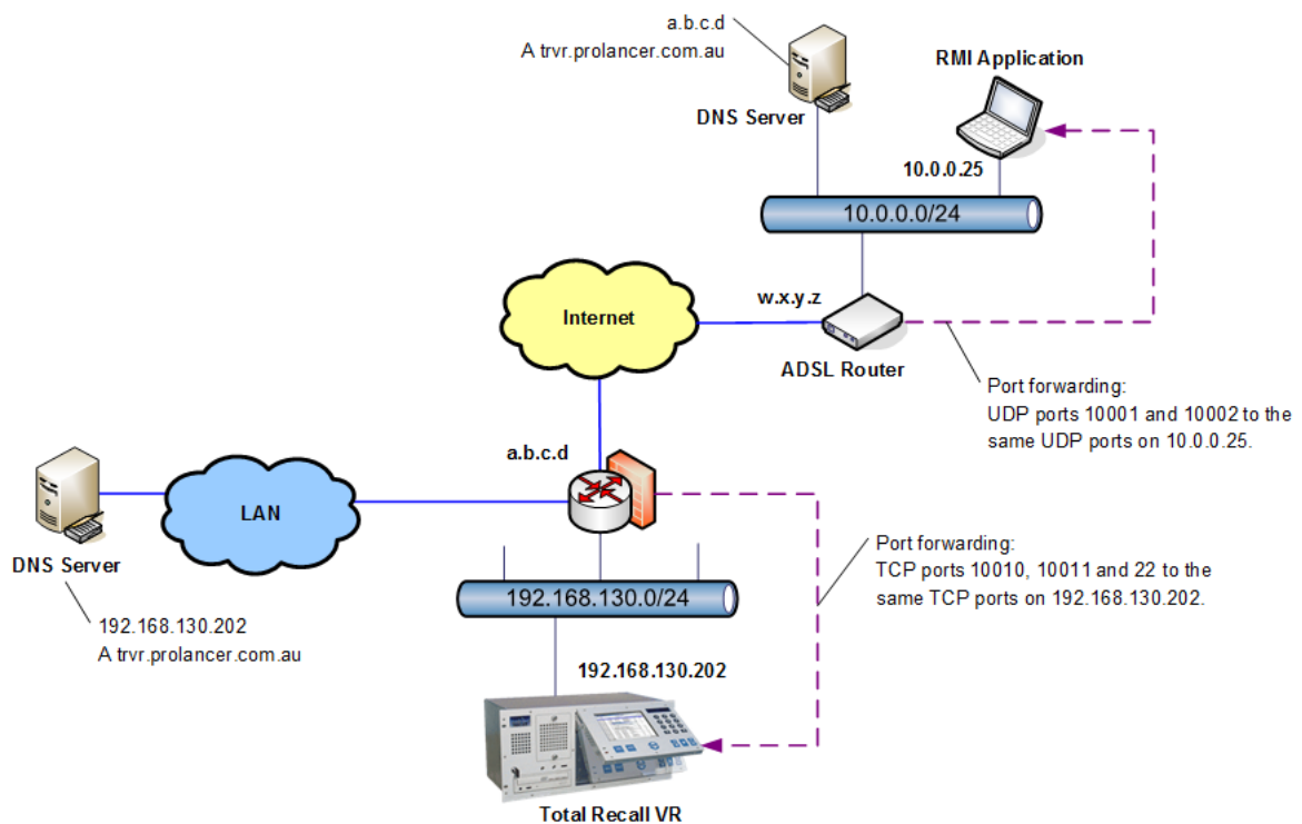
Figure 43: RMI Application through Firewall
