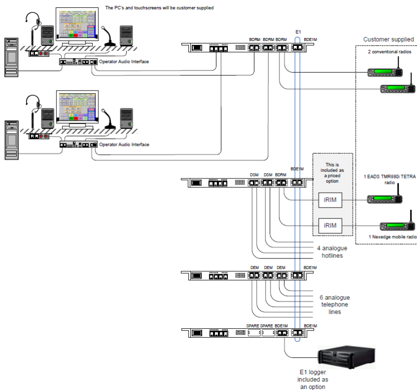
Figure 48: Typical Zetron DCS-5020 Solution
