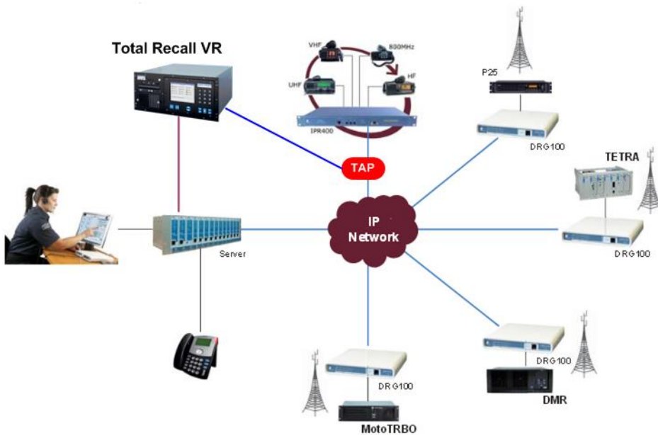
Figure 50: Total Recall VR working with DX-Altus
