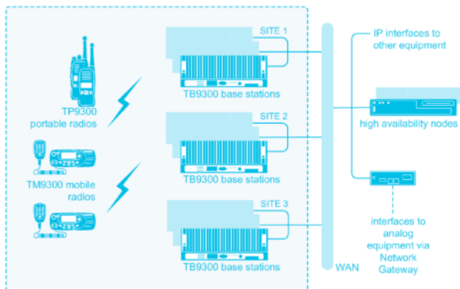
Figure 51: Typical Tait DMR Tier 3 Solution
