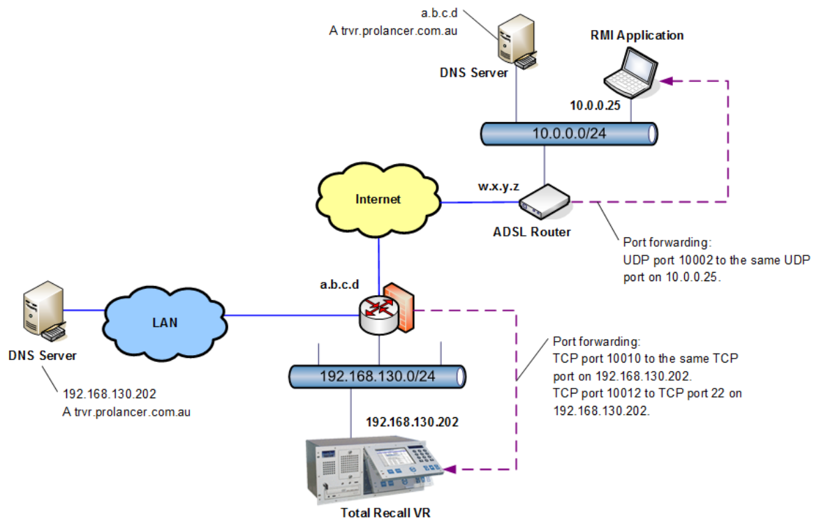
Figure 45: RMI Application through Firewall
