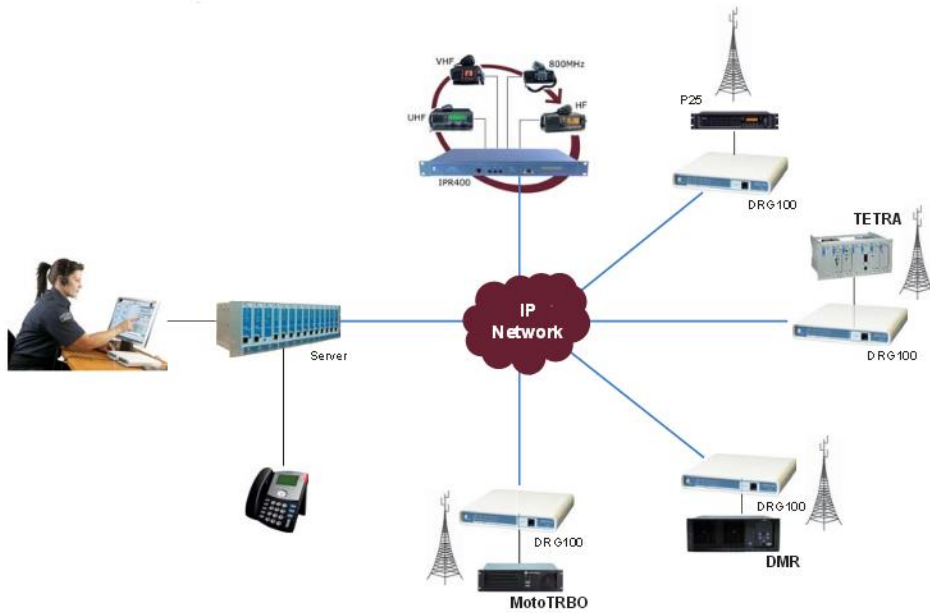
Figure 49: Typical DX-Altus Solution
